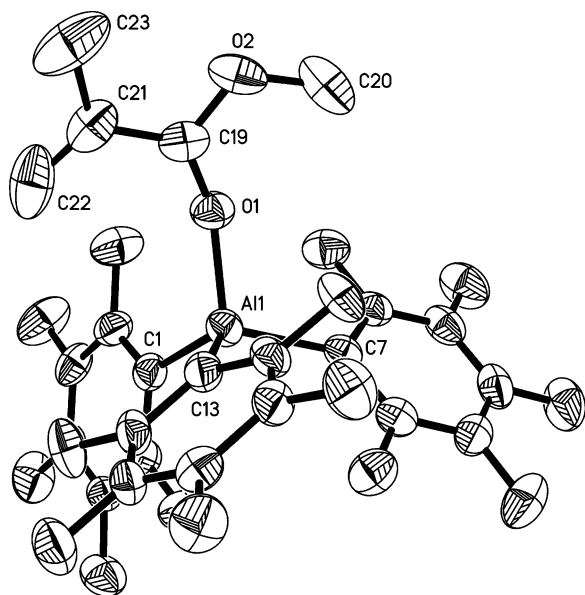
Figure 1. Molecular structure of the activated monomer \text{MMA}\cdot\text{Al}(\text{C}_6\text{F}_5)_3 ( 1 ).
