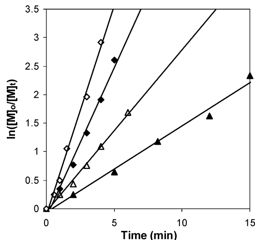
Figure 6. Semilogarithmic plots of \ln\{[\mathbf{M}]_0/[\mathbf{M}]_t\} versus time for the polymerization of MMA by 3 and \text{MeAl}(\text{BHT})_2 in toluene at 23 °C. Conditions: [\text{MMA}]_0 = 1.87 \text{ M} , [\mathbf{3}]_0 = 9.34 \text{ mM} , [\text{MeAl}(\text{BHT})_2]_0 = 9.34 \text{ mM} (▲), 18.7 mM (△); 28.0 mM (◆), 37.4 mM (◇).
