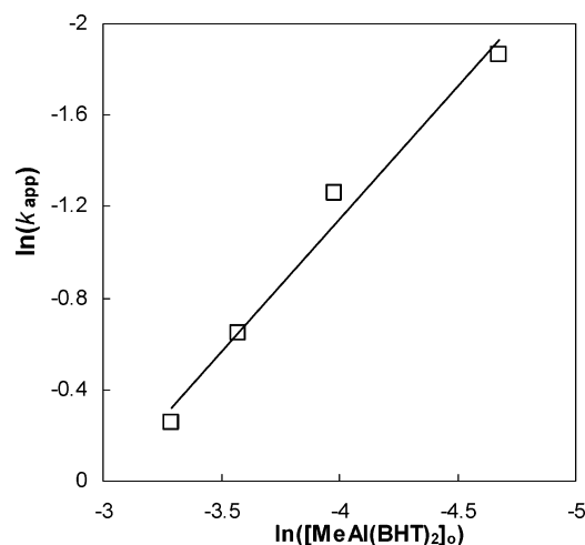
Figure 7. Plot of \ln(k_{\text{app}}) versus \ln\{[\text{MeAl}(\text{BHT})_2]_0\} for the MMA polymerization by 3 and \text{MeAl}(\text{BHT})_2 in toluene at 23 °C.
